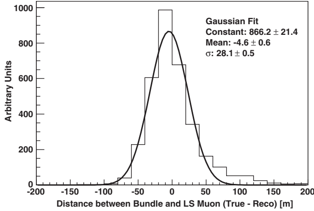
FIG. 7. The separation resolution of the bundle and LS muon reconstructions for Siblyll simulation at the final selection level.
