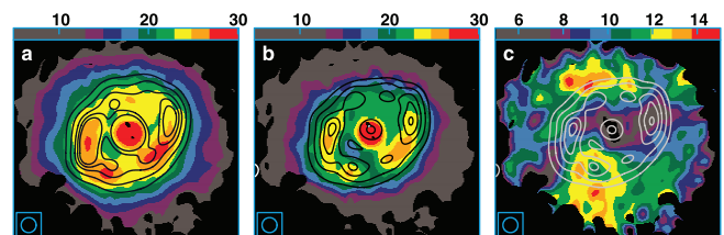
FIG. 5.—Magnetic maps of NGC 4736. (a) Total, (b) random, and (c) regular magnetic field strength (in \mu\text{G} ) in colors, with contours of (a) infrared 24 \mu\text{m} and (b, c) H \alpha emission.
