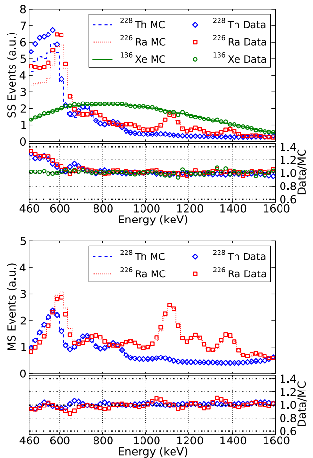
FIG. 1. Energy spectral agreement between data and MC simulation in SS (top) and MS (bottom) events. The comparison is presented between 460 keV and 1600 keV for two calibration sources, ^{228}\text{Th} and ^{226}\text{Ra} , deployed near the cathode of the detector for calibration runs. The background-subtracted ^{136}\text{Xe} - 2\nu\beta\beta spectrum is compared to MC only in SS events. A worsening of the agreement in SS \gamma -like spectra is observed for energies \lesssim 600 keV. This effect was considered in the searches as discussed in Sec. IV.
