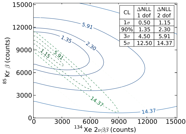
FIG. 4. Contour lines of the profile-likelihood ratio, \Delta\text{NLL} , scanned for the ^{85}\text{Kr } \beta and ^{134}\text{Xe } 2\nu\beta\beta components using two NLL functions. The blue solid lines were obtained using the same function as the ^{134}\text{Xe } 2\nu\beta\beta search, which accounts for all the systematic errors. The green dashed lines were evaluated without consideration of the normalization errors. The table shows \Delta\text{NLL} values of various C.L.'s for 1 and 2 d.o.f.
