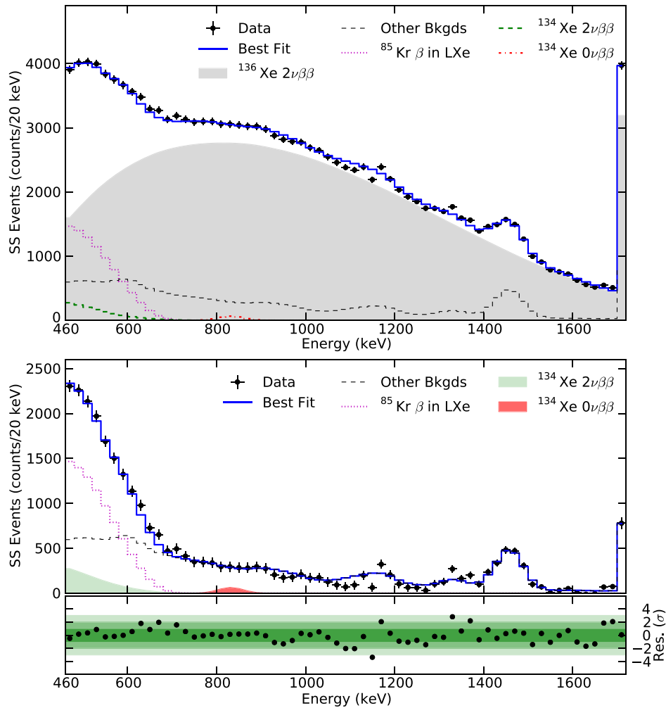
FIG. 3. The top plot shows the SS energy projection for the results of the ^{134}\text{Xe} - 2\nu\beta\beta analysis, using the fitted central values. While the 0\nu\beta\beta search is performed in a separate fit with a higher energy threshold, it is overlaid here for comparison since the backgrounds at these energies are the same. The last bin is the summed contents of all bins between 1700 keV and 9800 keV. The middle plot shows the same results, where the ^{136}\text{Xe} - 2\nu\beta\beta component is subtracted from data and best-fit values. The bottom plot presents the residuals between data and best fit normalized to the Poisson error.
