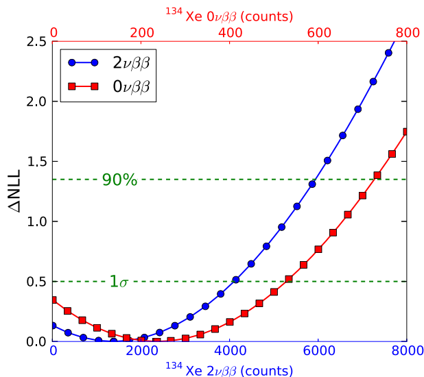
FIG. 2. Profile-likelihood ratio, \Delta\text{NLL} , for ^{134}\text{Xe} 2\nu\beta\beta and 0\nu\beta\beta . The dashed lines represent the 1\sigma and 90% C.L.'s, assuming the validity of Wilks's theorem [22,23]. The latter intersects the profile curves at 5900 and 730 counts for 2\nu\beta\beta and 0\nu\beta\beta , respectively.
