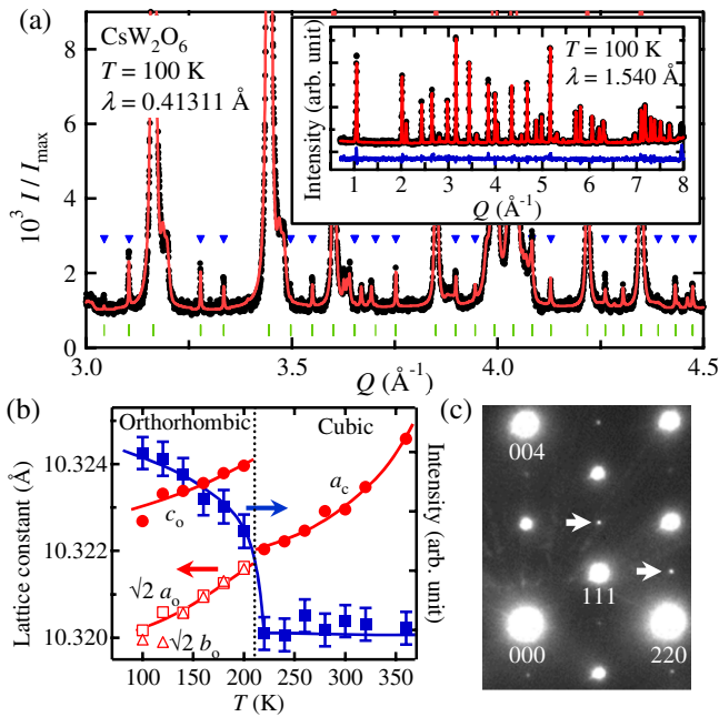
FIG. 2 (color online). (a) Portion of the Rietveld fit of the synchrotron x-ray powder diffraction pattern for \text{CsW}_2\text{O}_6 at 100 K. The triangles mark the superlattice reflections. The inset shows the Rietveld fit of the neutron powder diffraction data at 100 K. (b) The temperature dependence of lattice constants and the integrated intensities of superlattice peak with index (111) in synchrotron x-ray data. The solid lines are guides for the eyes. (c) Electron diffraction pattern for \text{CsW}_2\text{O}_6 at 100 K with the incident beam parallel to the [110] cubic zone axis. The spots pointed by arrows violate the extinction rules for the F centering of cubic unit cell.
