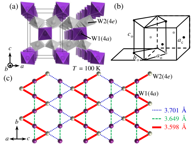
FIG. 3 (color online). (a) \text{WO}_6 network at 100 K showing the formation of one-dimensional chains. (b) The relation between the cubic cell and orthorhombic cell. (c) W networks on Kagome lattice at 100 K, where W-W bonds with different lengths are shown differently.
