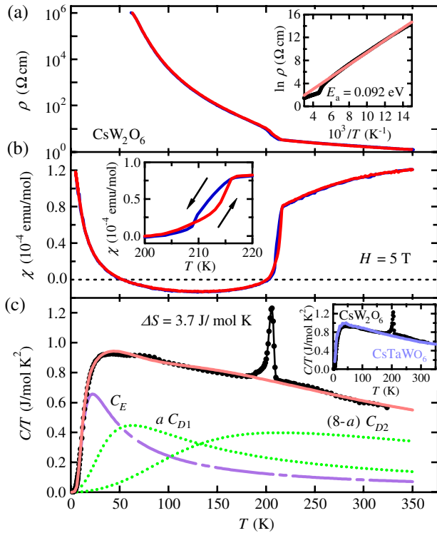
FIG. 1 (color online). Temperature dependence of (a) electrical resistivity, (b) magnetic susceptibility, and (c) specific heat divided by temperature of \text{CsW}_2\text{O}_6 . C/T(T) data are plotted with the fit (solid line) consisting of an Einstein phonon (broken line) and two Debye phonons (dotted line) as described in Ref. [16]. Inset in (a) Arrhenius plot [ \ln \rho(T) vs T^{-1} ] of \text{CsW}_2\text{O}_6 . Inset in (b) Enlarged regions of magnetic susceptibility showing the hysteresis associated with a first order transition. (c) Comparison of C/T(T) between \text{CsTaWO}_6 (solid line) from Ref. [15] and \text{CsW}_2\text{O}_6 (dots).
