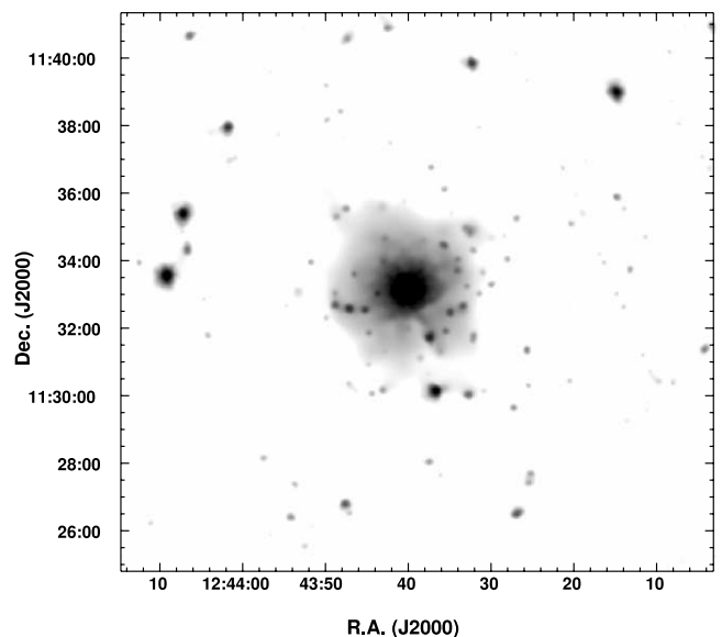
FIG. 2.—Adaptively smoothed XMM-Newton image of NGC 4649 using MOS1, MOS2, and PN data, cleaned of background flares and corrected for exposure and background. The gray scale is logarithmic and ranges from 2.2 \times 10^{-5} to 4.7 \times 10^{-4} counts s -1 pixel -1 .
